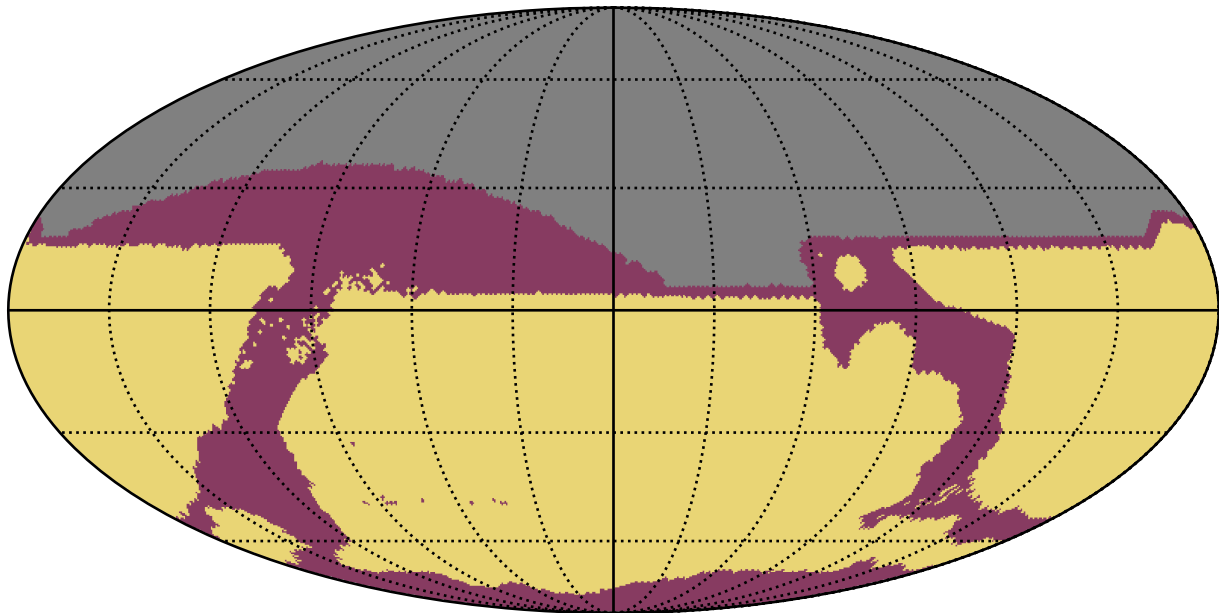
ddf_acor_sf30_lsf40_lsr10_v3.4_10yrs All sky: RapidRevisits
