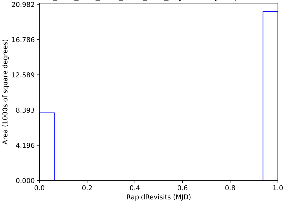
ddf_acor_sf30_lsf40_lsr10_v3.4_10yrs All sky: RapidRevisits
