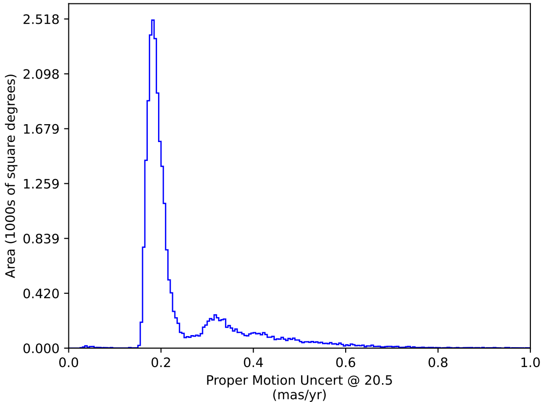
ddf_acor_sf30_lsf40_lsr10_v3.4_10yrs All sky: Proper Motion Uncert @ 20.5
