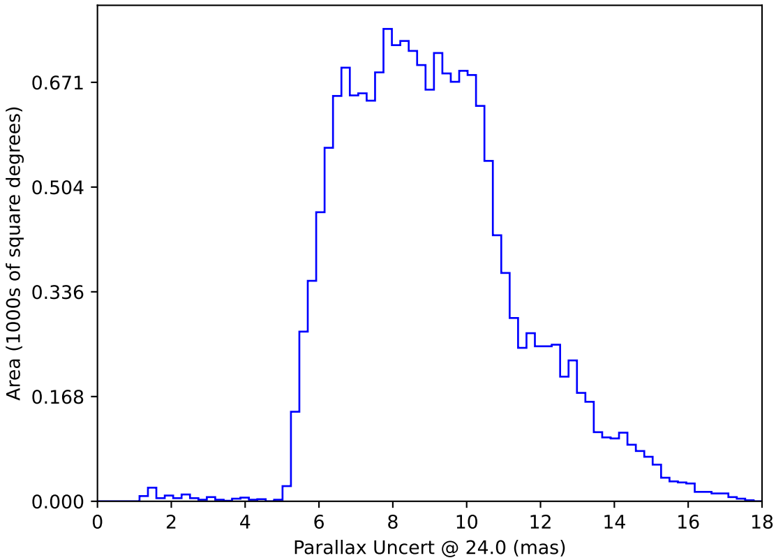
ddf_acor_sf30_lsf40_lsr10_v3.4_10yrs WFD: Parallax Uncert @ 24.0
