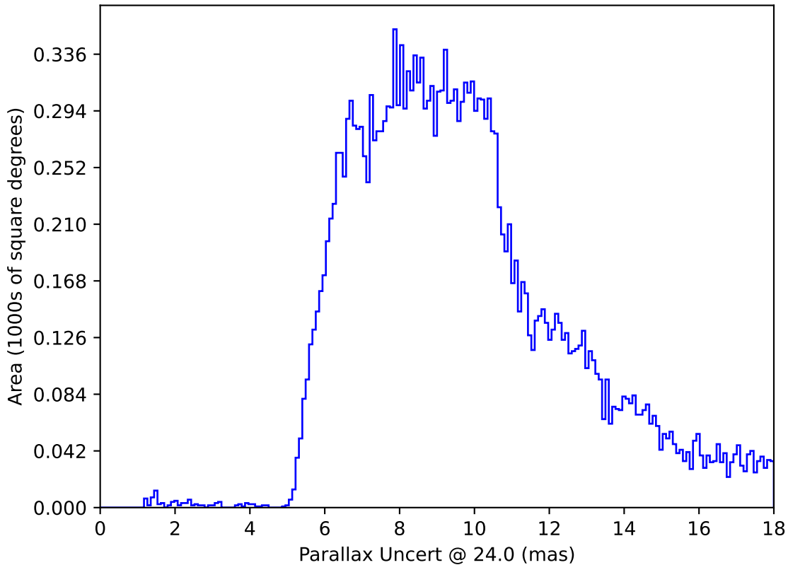
ddf_acor_sf30_lsf40_lsr10_v3.4_10yrs All sky: Parallax Uncert @ 24.0
