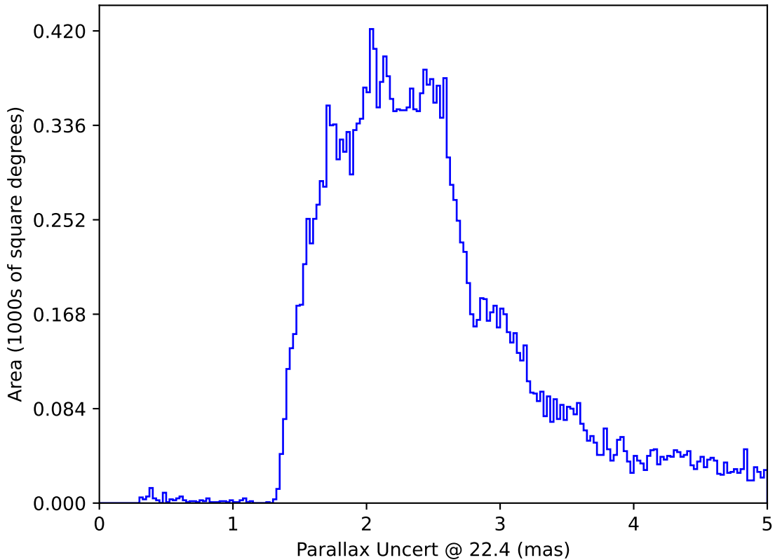
ddf_acor_sf30_lsf40_lsr10_v3.4_10yrs All sky: Parallax Uncert @ 22.4
