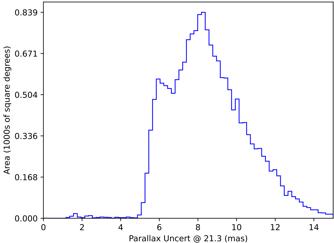
ddf_acor_sf30_lsf40_lsr10_v3.4_10yrs WFD y band only: Parallax Uncert @ 21.3
