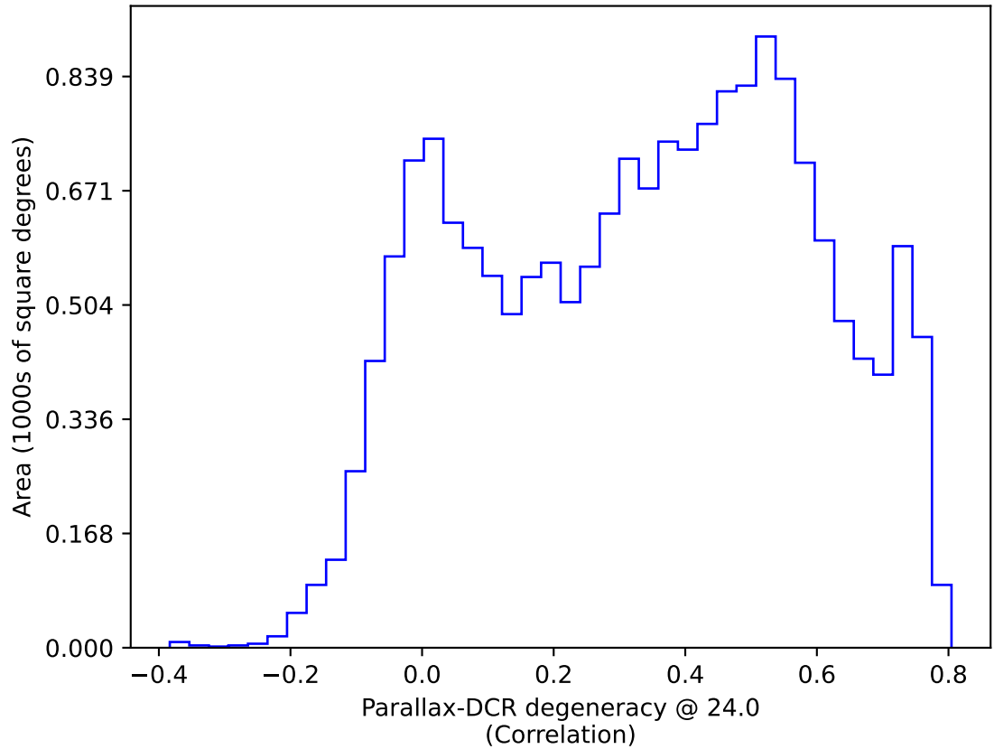
ddf_acor_sf30_lsf40_lsr10_v3.4_10yrs WFD: Parallax-DCR degeneracy @ 24.0
