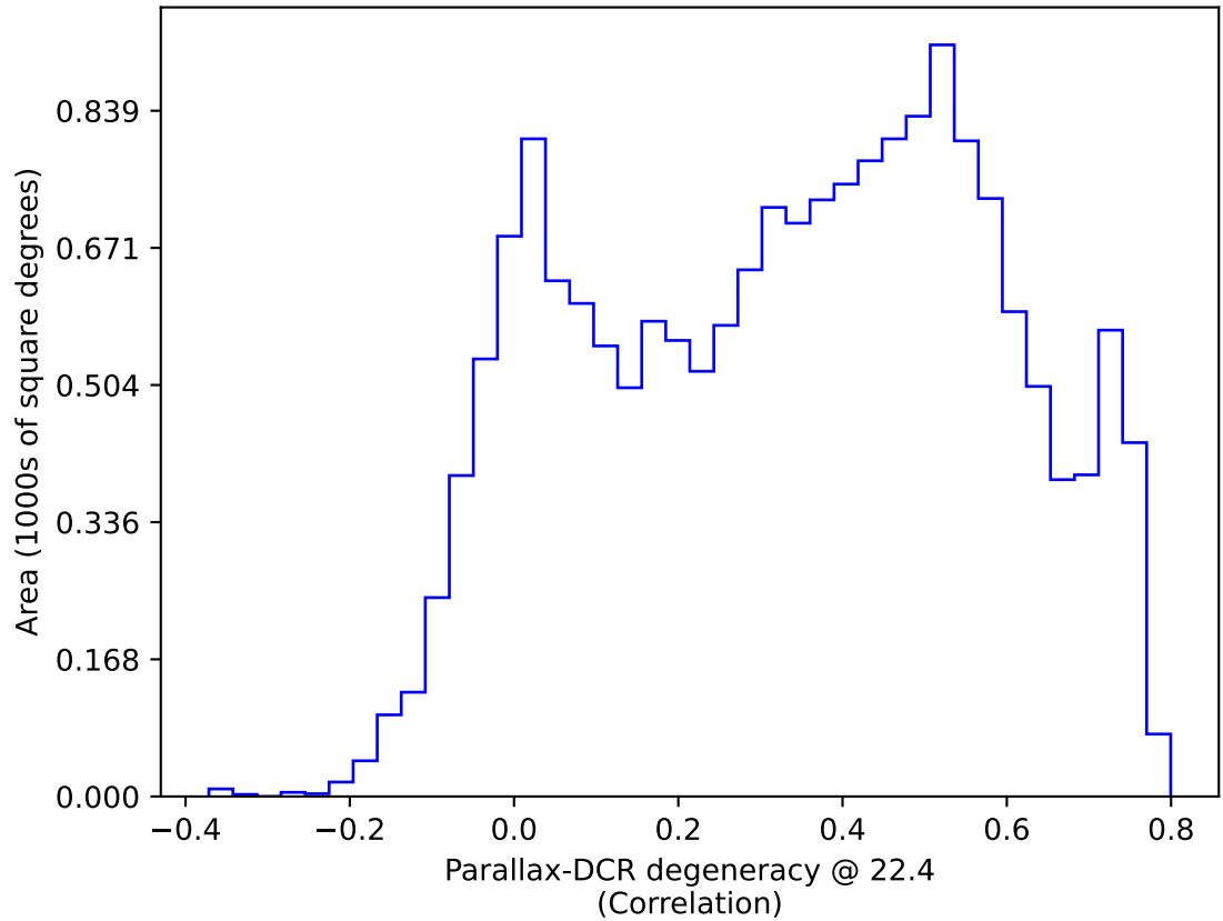
ddf_acor_sf30_lsf40_lsr10_v3.4_10yrs WFD: Parallax-DCR degeneracy @ 22.4
