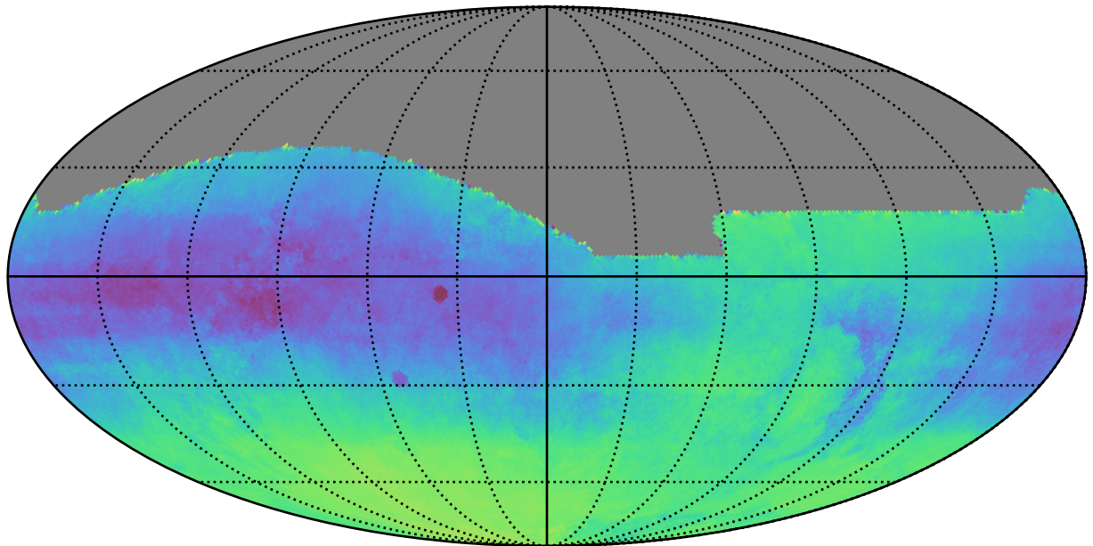
ddf_acor_sf30_lsf40_lsr10_v3.4_10yrs All sky: Parallax-DCR degeneracy @ 22.4
