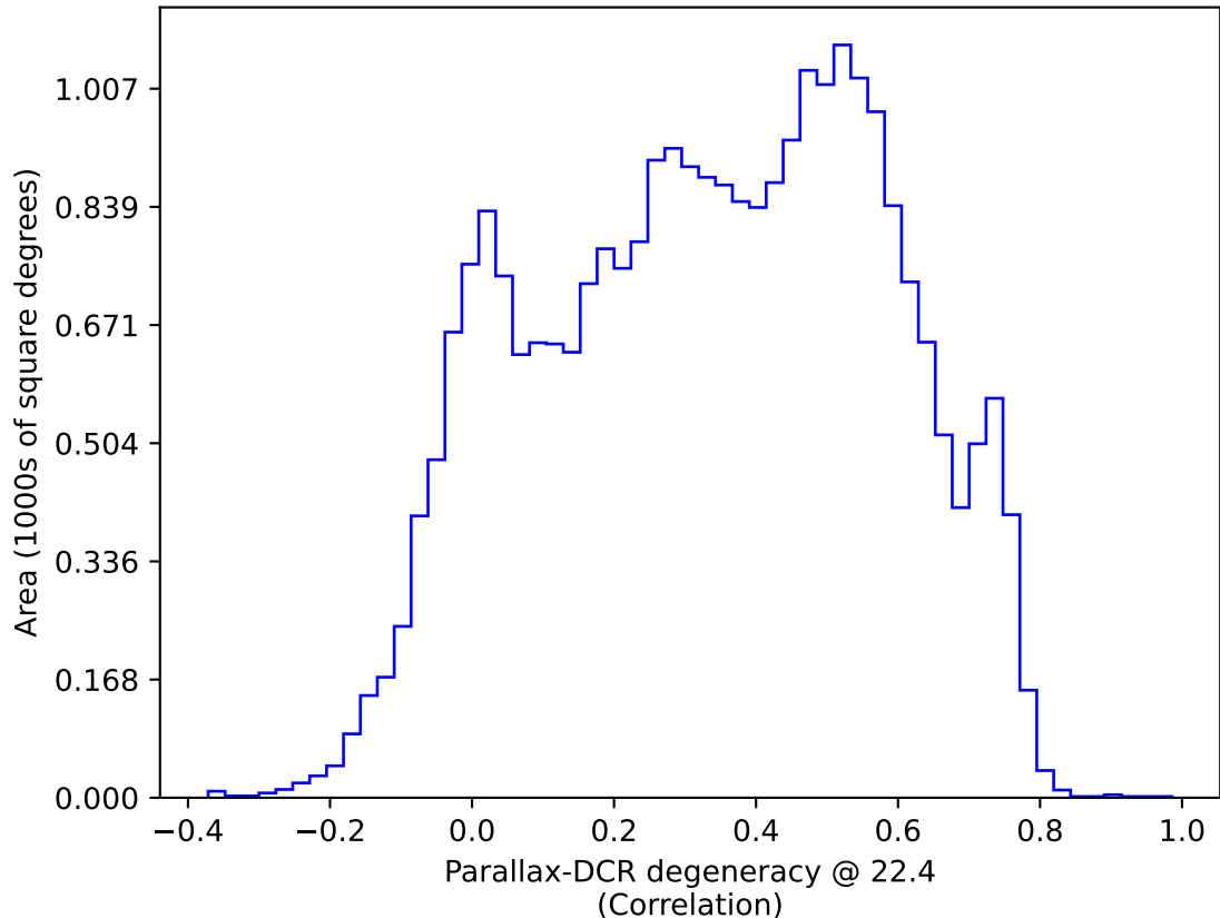
ddf_acor_sf30_lsf40_lsr10_v3.4_10yrs All sky: Parallax-DCR degeneracy @ 22.4
