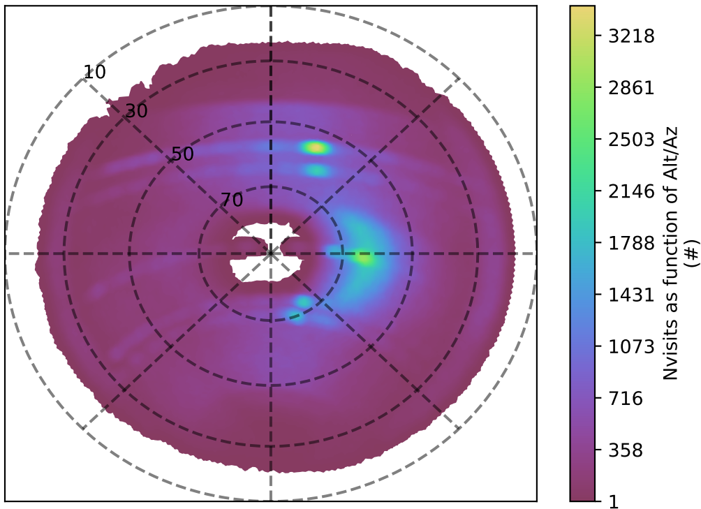
ddf_acor_sf30_lsf40_lsr10_v3.4_10yrs z band: Nvisits as function of Alt/Az
