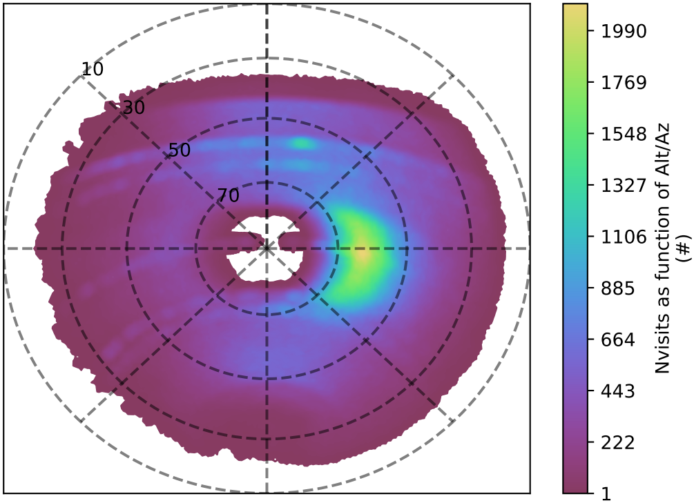
ddf_acor_sf30_lsf40_lsr10_v3.4_10yrs y band: Nvisits as function of Alt/Az
