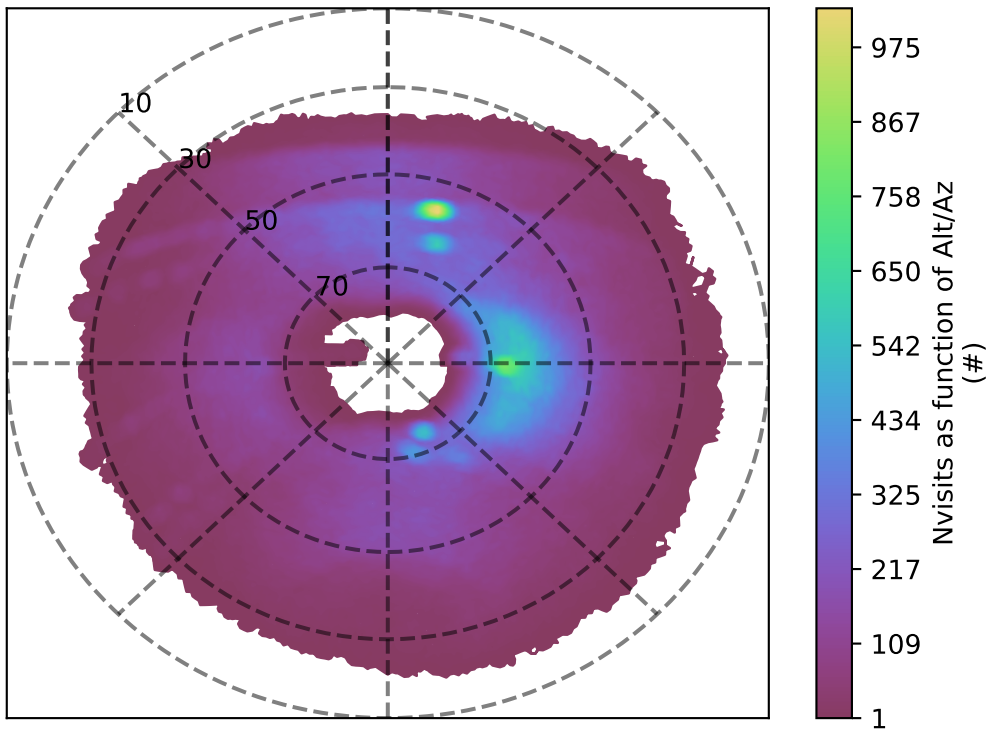
ddf_acor_sf30_lsf40_lsr10_v3.4_10yrs u band: Nvisits as function of Alt/Az
