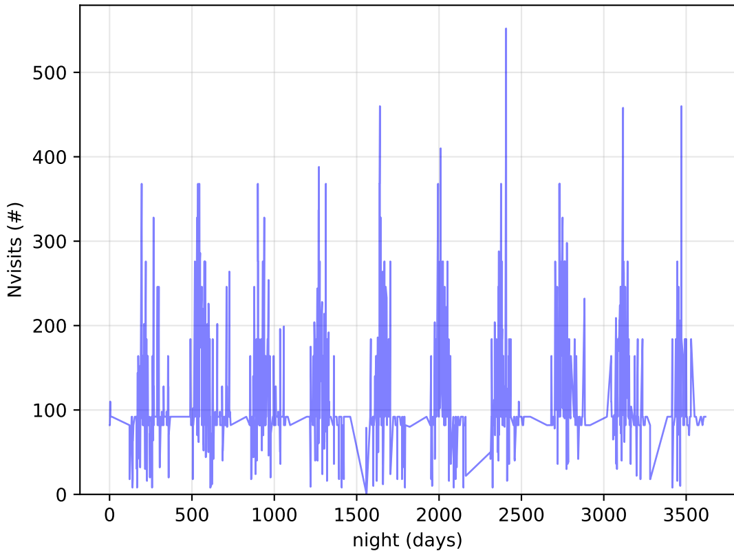
ddf_acor_sf30_ls40_lsr10_v3.4_10yrs DDF: Nvisits
