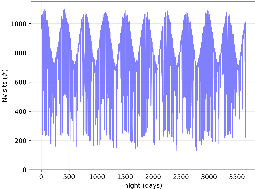
ddf_acor_sf30_lsf40_lsr10_v3.4_10yrs All visits: Nvisits
