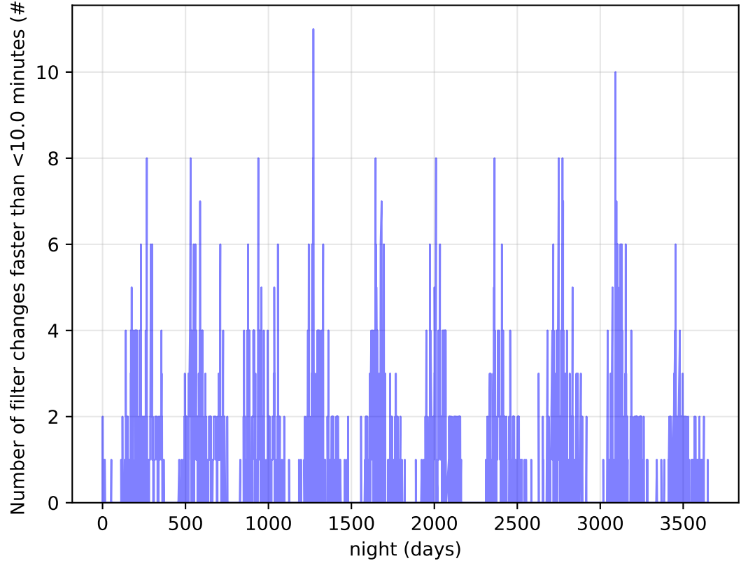
ddf_acor_sf30_Isf40_Isr10_v3.4_10yrs Per Night: Number of filter changes faster than <10.0 minutes
