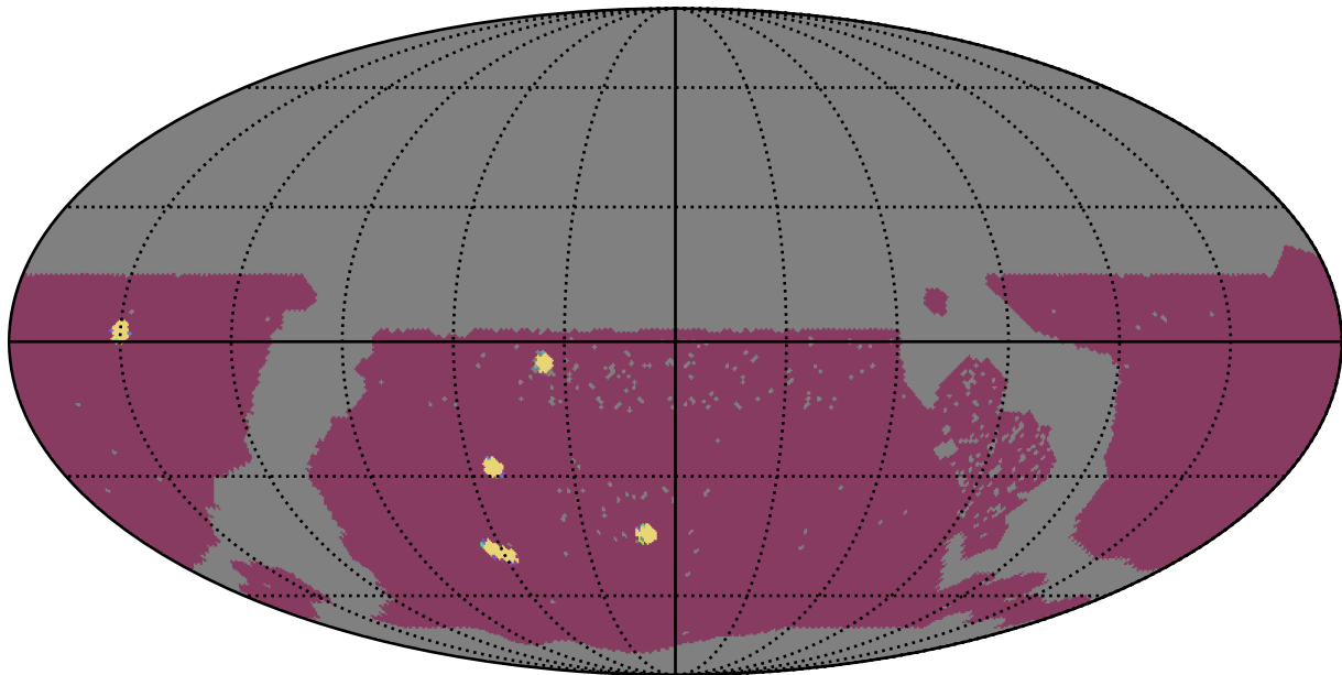
ddf_acor_sf30_lsf40_lsr10_v3.4_10yrs WFD: NumberOfQuickRevisits
