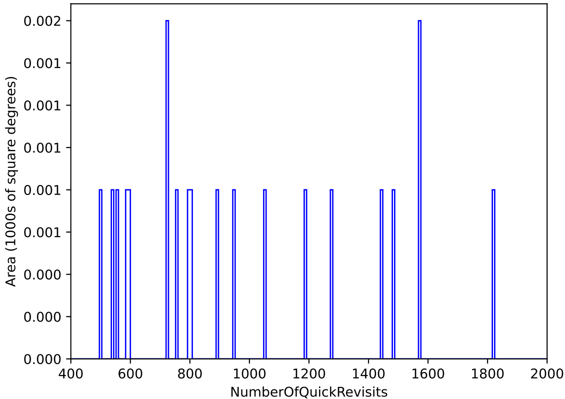
ddf_acor_sf30_Isf40_Isr10_v3.4_10yrs All sky: NumberOfQuickRevisits
