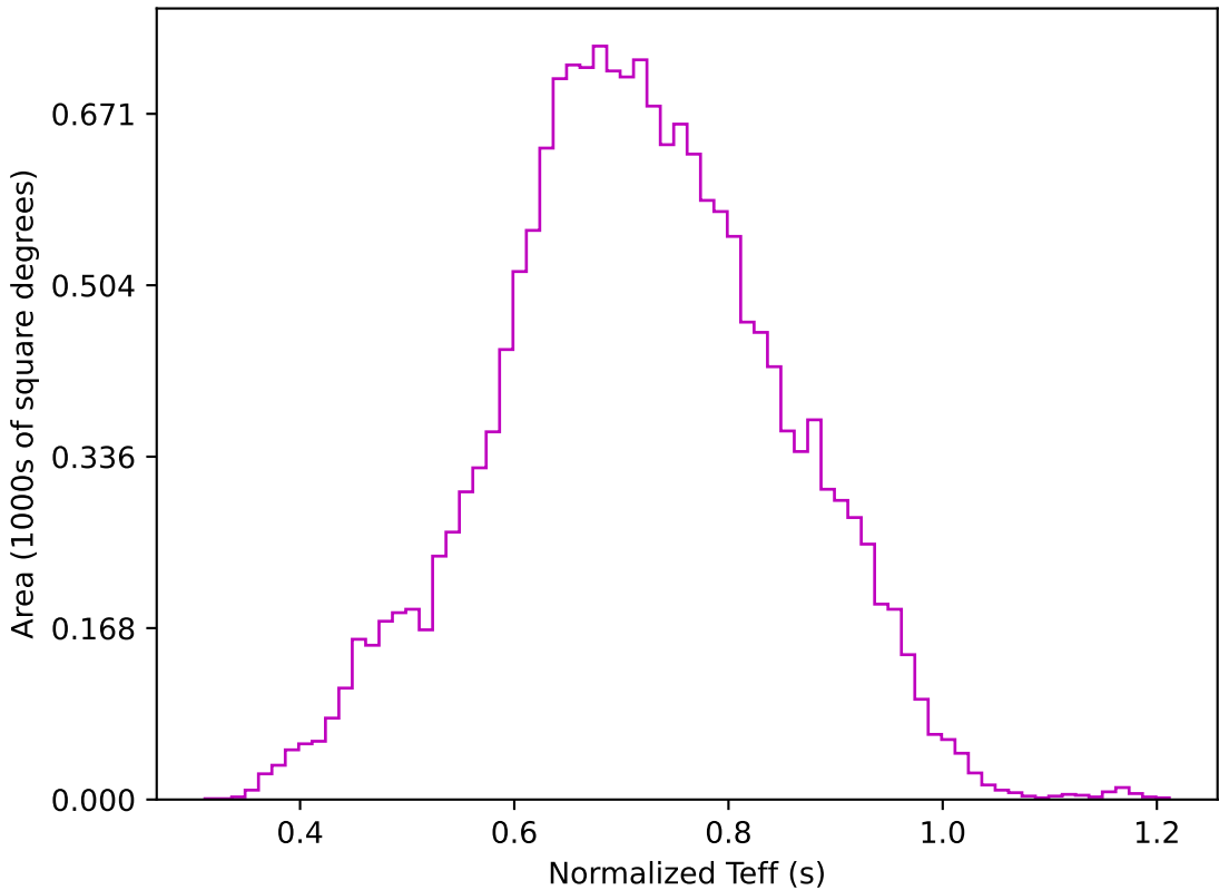
ddf_acor_sf30_lsf40_lsr10_v3.4_10yrs WFD z band: Normalized Teff
