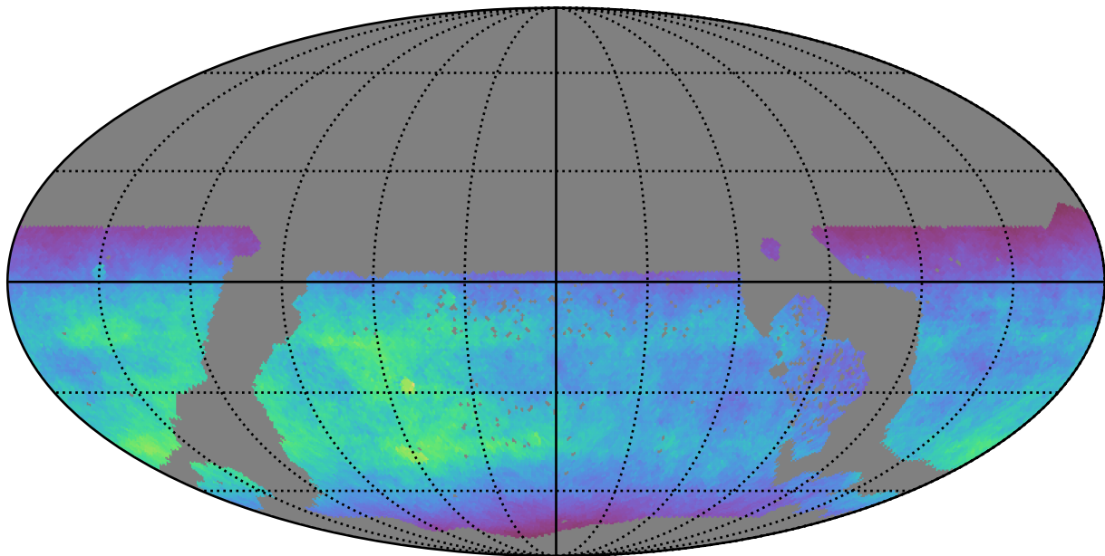
ddf_acor_sf30_lsf40_lsr10_v3.4_10yrs WFD y band: Normalized Teff
