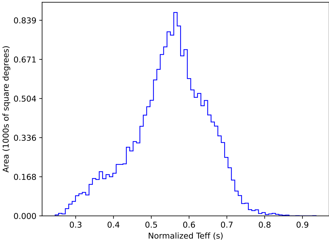
ddf_acor_sf30_lsf40_lsr10_v3.4_10yrs WFD y band: Normalized Teff
