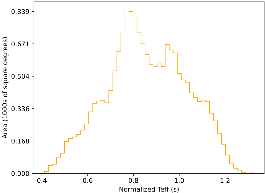
ddf_acor_sf30_lsf40_lsr10_v3.4_10yrs WFD r band: Normalized Teff
