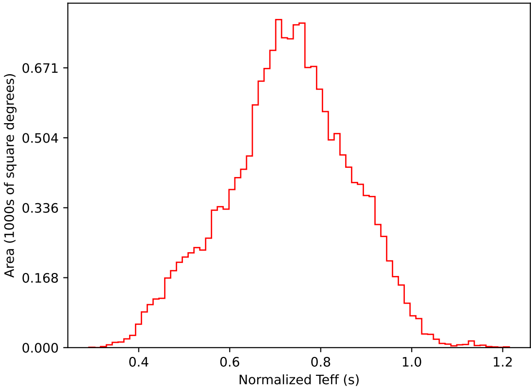
ddf_acor_sf30_lsf40_lsr10_v3.4_10yrs WFD i band: Normalized Teff
