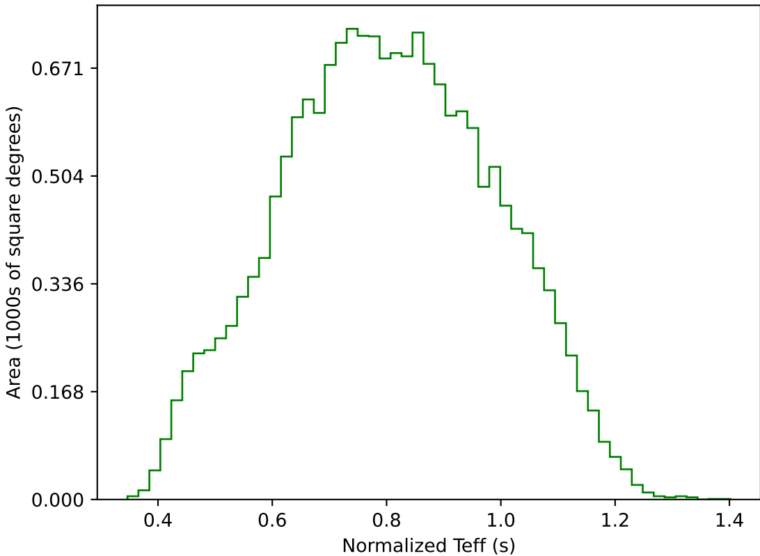
ddf_acor_sf30_lsf40_lsr10_v3.4_10yrs WFD g band: Normalized Teff
