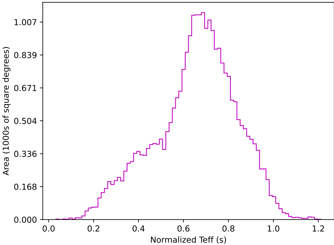
ddf_acor_sf30_lsf40_lsr10_v3.4_10yrs All sky z band: Normalized Teff
