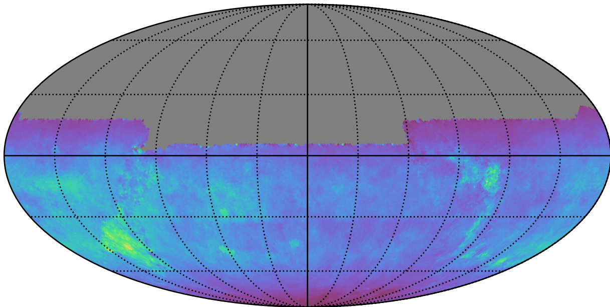
ddf_acor_sf30_lsf40_lsr10_v3.4_10yrs All sky u band: Normalized Teff
