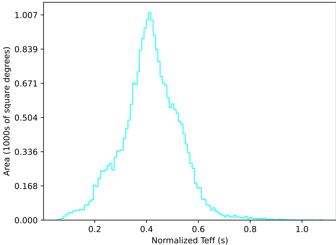
ddf_acor_sf30_lsf40_lsr10_v3.4_10yrs All sky u band: Normalized Teff
