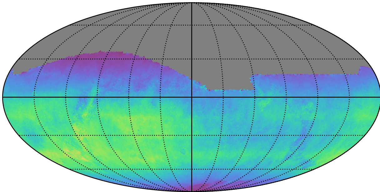
ddf_acor_sf30_lsf40_lsr10_v3.4_10yrs All sky r band: Normalized Teff
