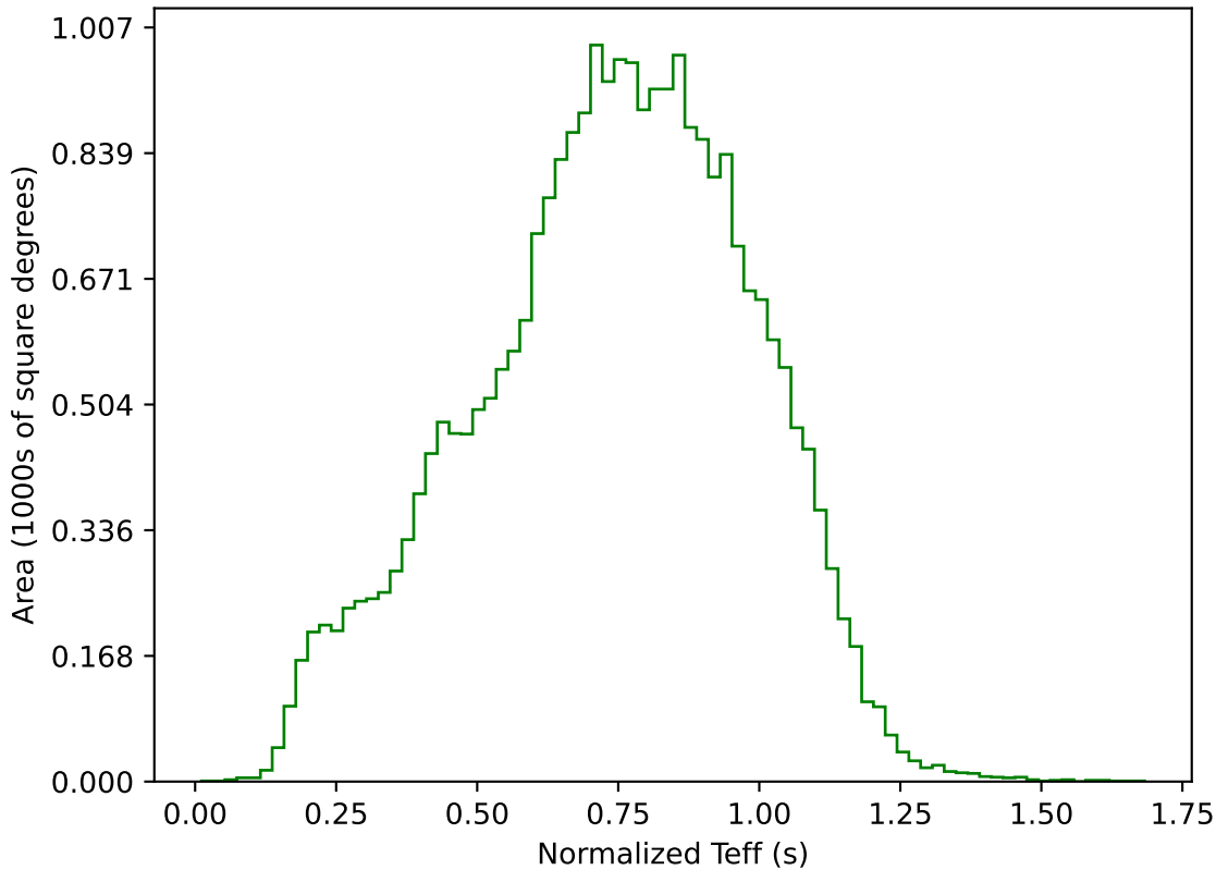
ddf_acor_sf30_lsf40_lsr10_v3.4_10yrs All sky g band: Normalized Teff
