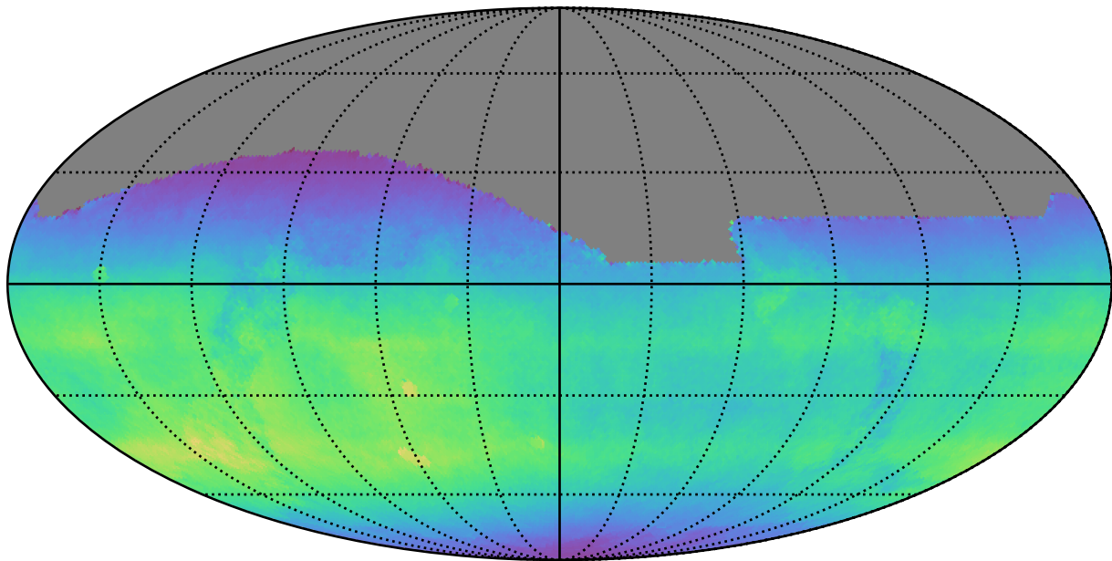
ddf_acor_sf30_lsf40_lsr10_v3.4_10yrs All sky all bands: Normalized Teff
