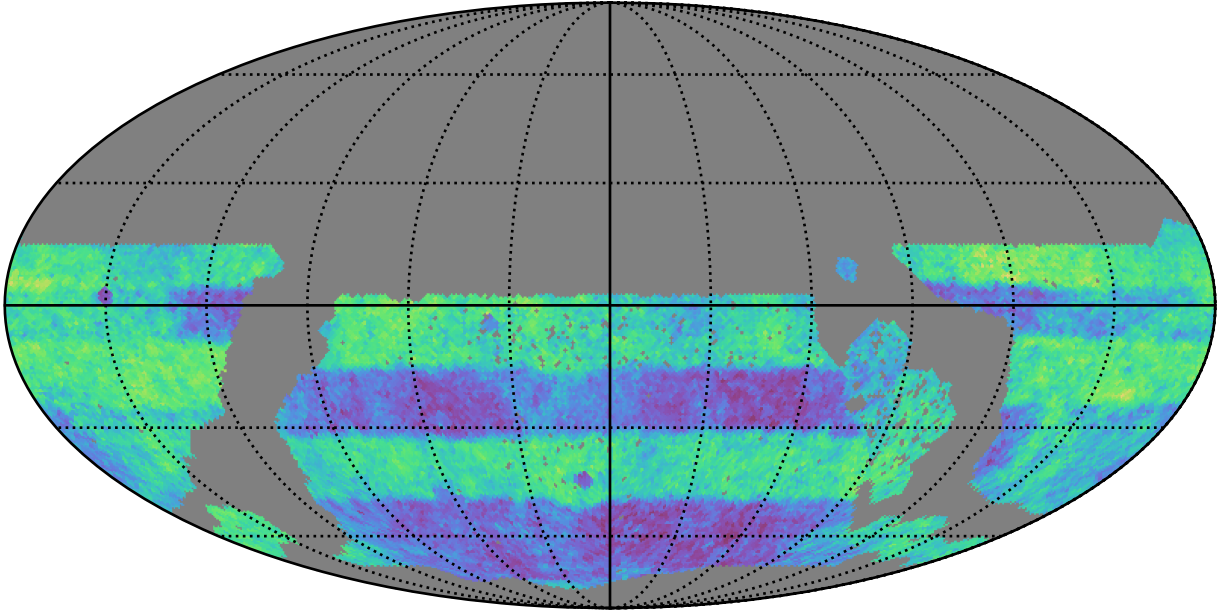
ddf_acor_sf30_lsf40_lsr10_v3.4_10yrs WFD: Normalized Proper Motion Uncert @ 24.0
