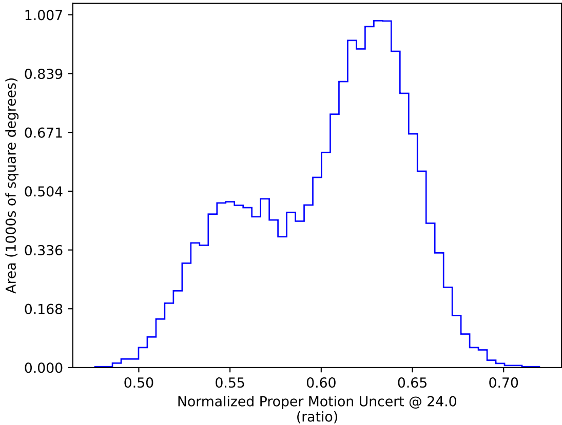
ddf_acor_sf30_lsf40_lsr10_v3.4_10yrs WFD: Normalized Proper Motion Uncert @ 24.0
