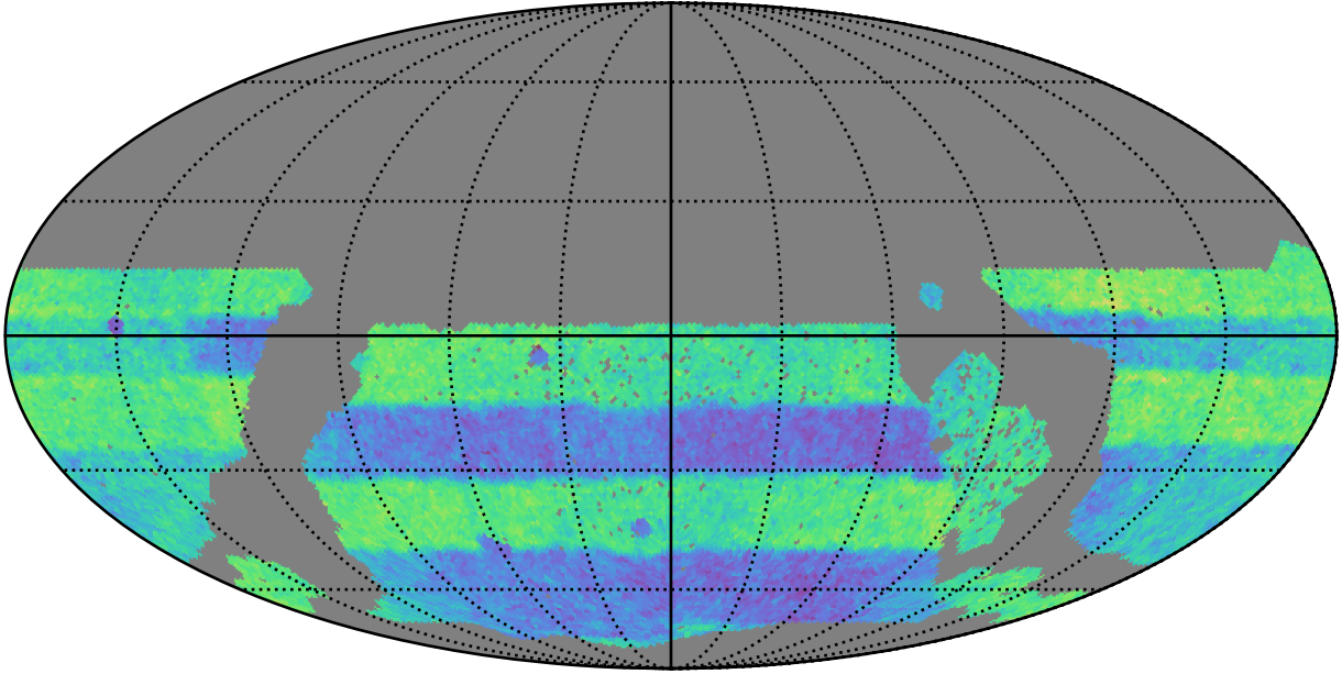
ddf_acor_sf30_lsf40_lsr10_v3.4_10yrs WFD: Normalized Proper Motion Uncert @ 20.5
