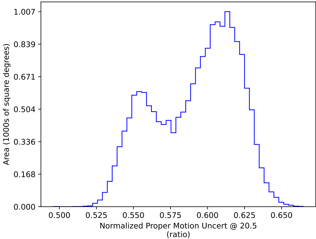
ddf_acor_sf30_lsf40_lsr10_v3.4_10yrs WFD: Normalized Proper Motion Uncert @ 20.5
