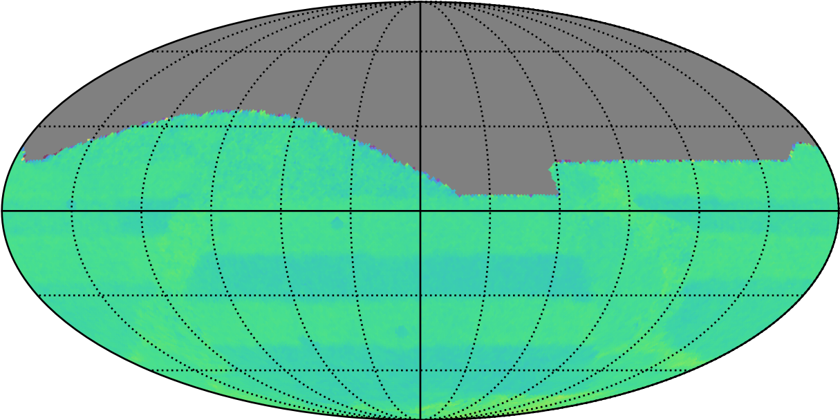
ddf_acor_sf30_lsf40_lsr10_v3.4_10yrs All sky: Normalized Proper Motion Uncert @ 20.5
