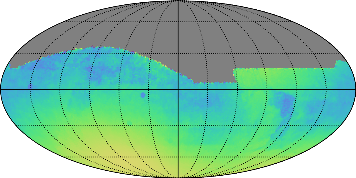
ddf_acor_sf30_lsf40_lsr10_v3.4_10yrs All sky: Normalized Parallax Uncert @ 24.0
