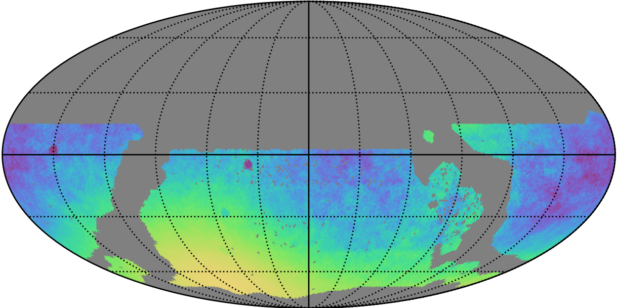
ddf_acor_sf30_lsf40_lsr10_v3.4_10yrs WFD y band only: Normalized Parallax Uncert @ 21.3
