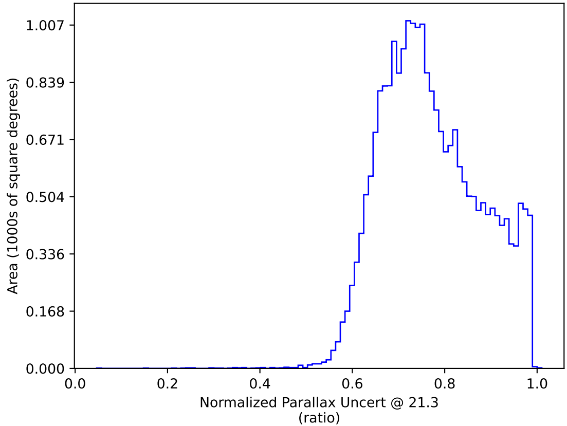
ddf_acor_sf30_lsf40_lsr10_v3.4_10yrs All sky y band only: Normalized Parallax Uncert @ 21.3
