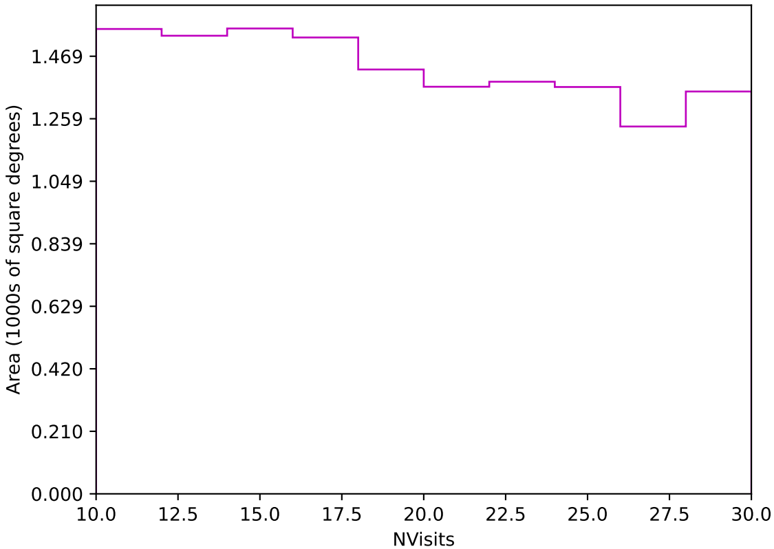
ddf_acor_sf30_lsf40_lsr10_v3.4_10yrs Yr 3-4 z band: NVisits
