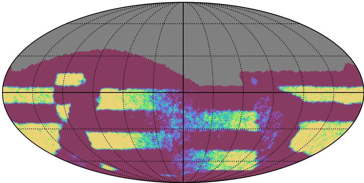
ddf_acor_sf30_lsf40_lsr10_v3.4_10yrs Yr 3-4 all bands: NVisits
