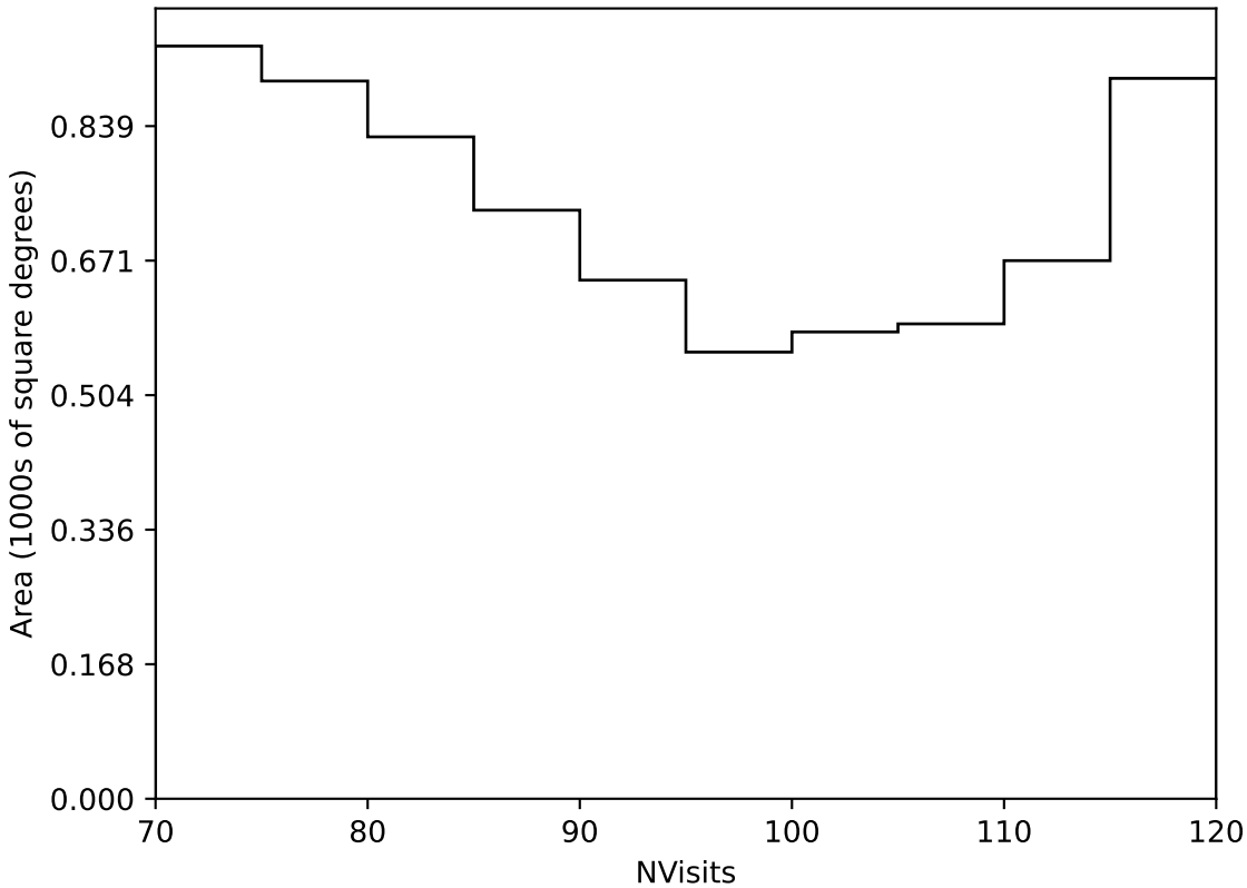
ddf_acor_sf30_lsf40_lsr10_v3.4_10yrs Yr 3-4 all bands: NVisits
