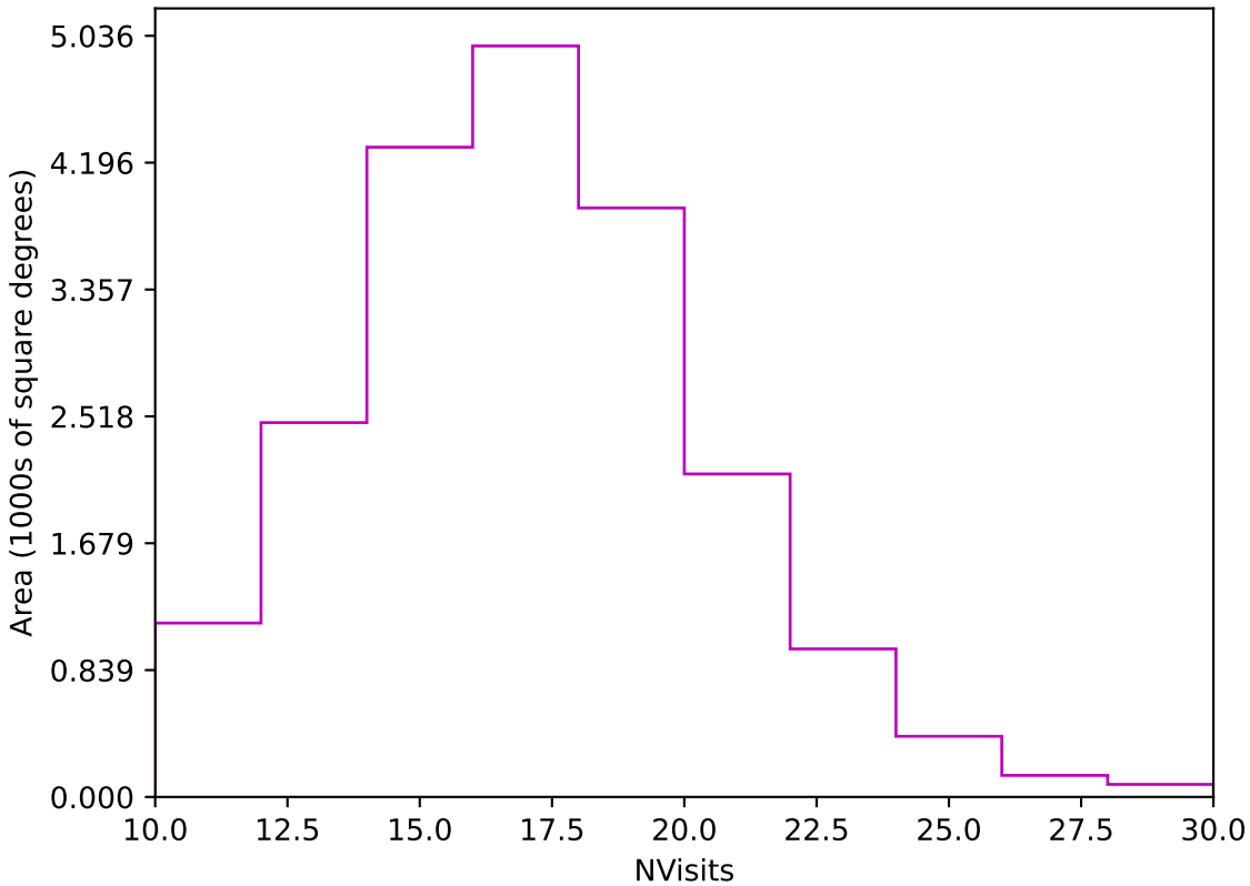
ddf_acor_sf30_lsf40_lsr10_v3.4_10yrs Yr 1 z band: NVisits
