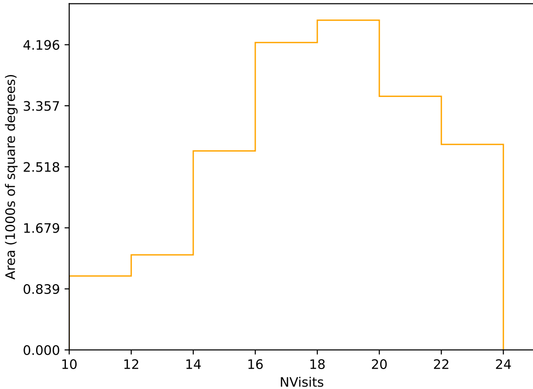
ddf_acor_sf30_lsf40_lsr10_v3.4_10yrs Yr 1 r band: NVisits
