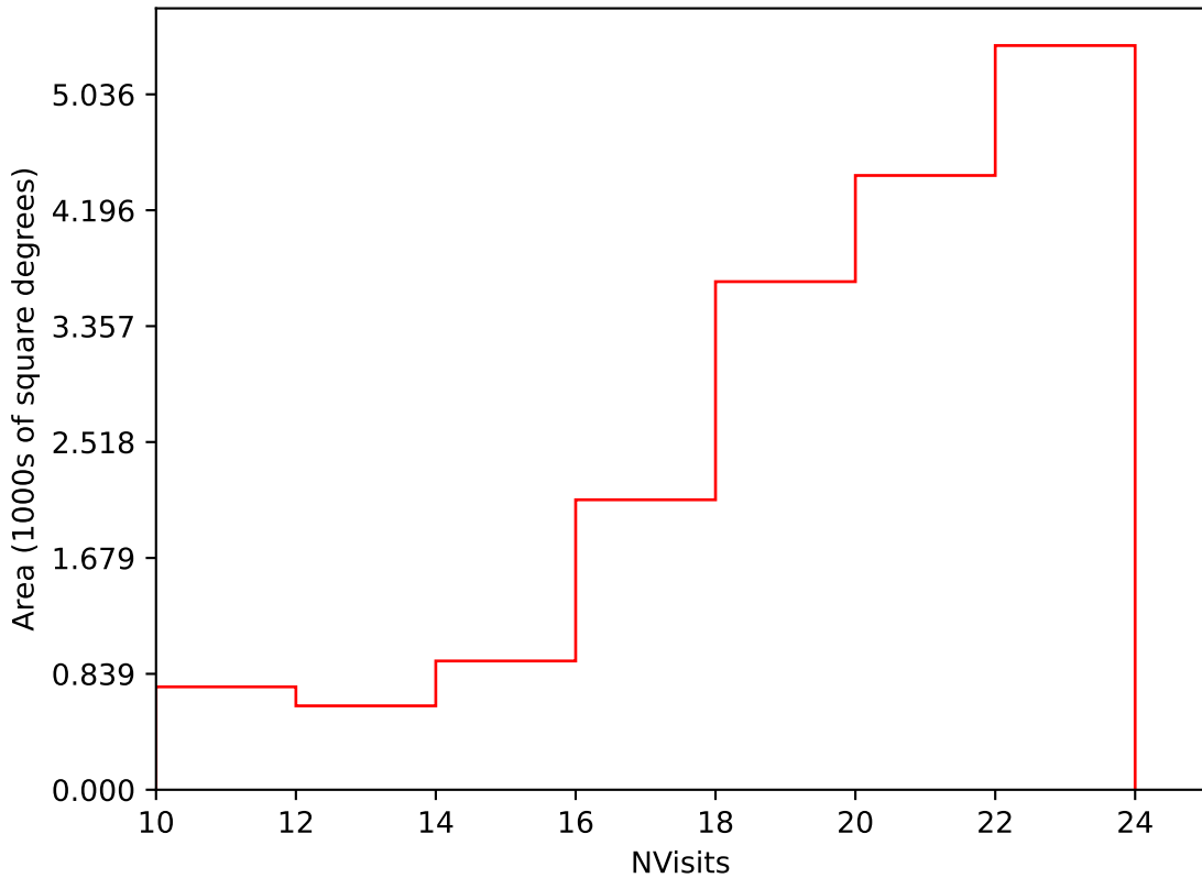
ddf_acor_sf30_lsf40_lsr10_v3.4_10yrs Yr 1 i band: NVisits
