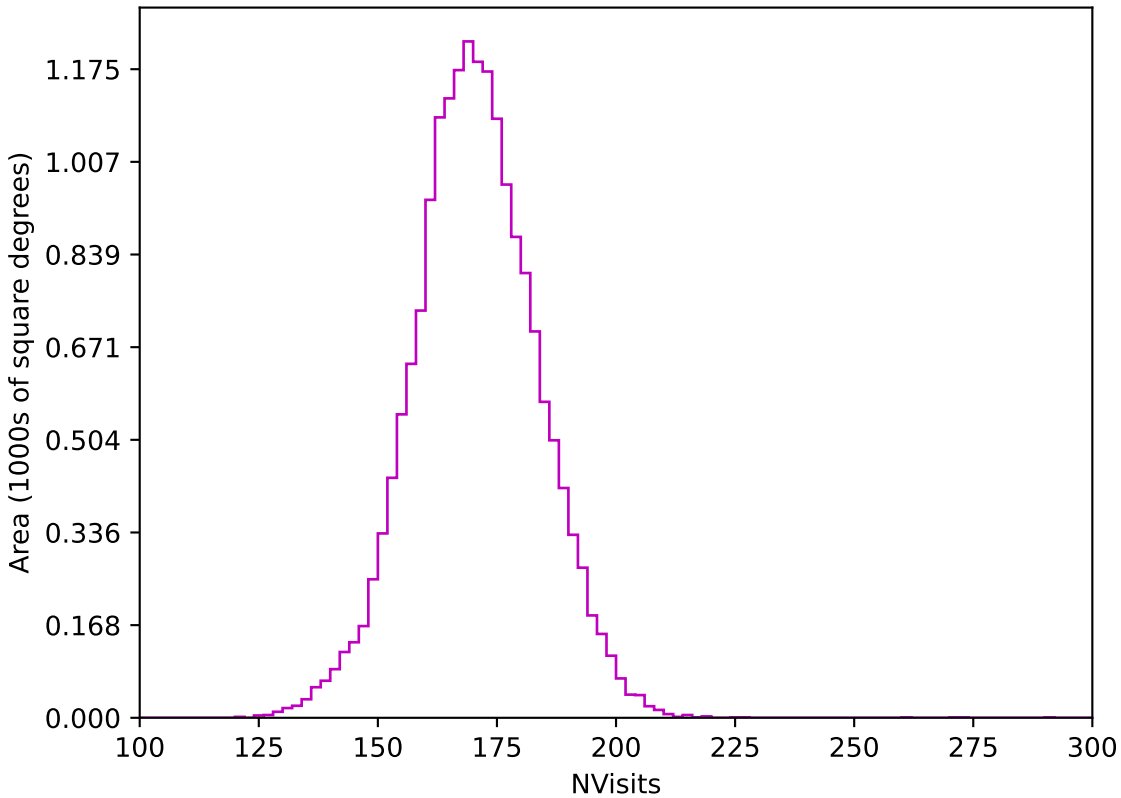
ddf_acor_sf30_lsf40_lsr10_v3.4_10yrs WFD z band: NVisits
