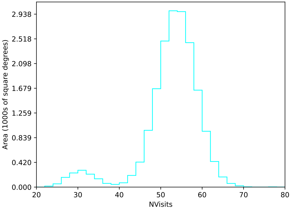
ddf_acor_sf30_lsf40_lsr10_v3.4_10yrs WFD u band: NVisits
