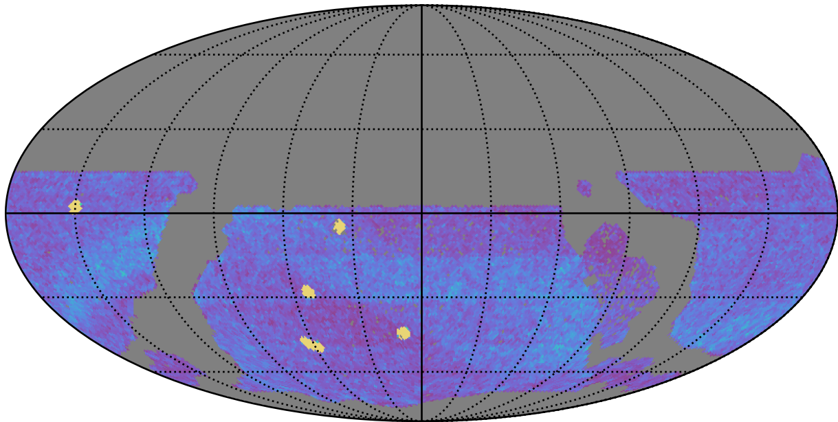
ddf_acor_sf30_lsf40_lsr10_v3.4_10yrs WFD all bands: NVisits
