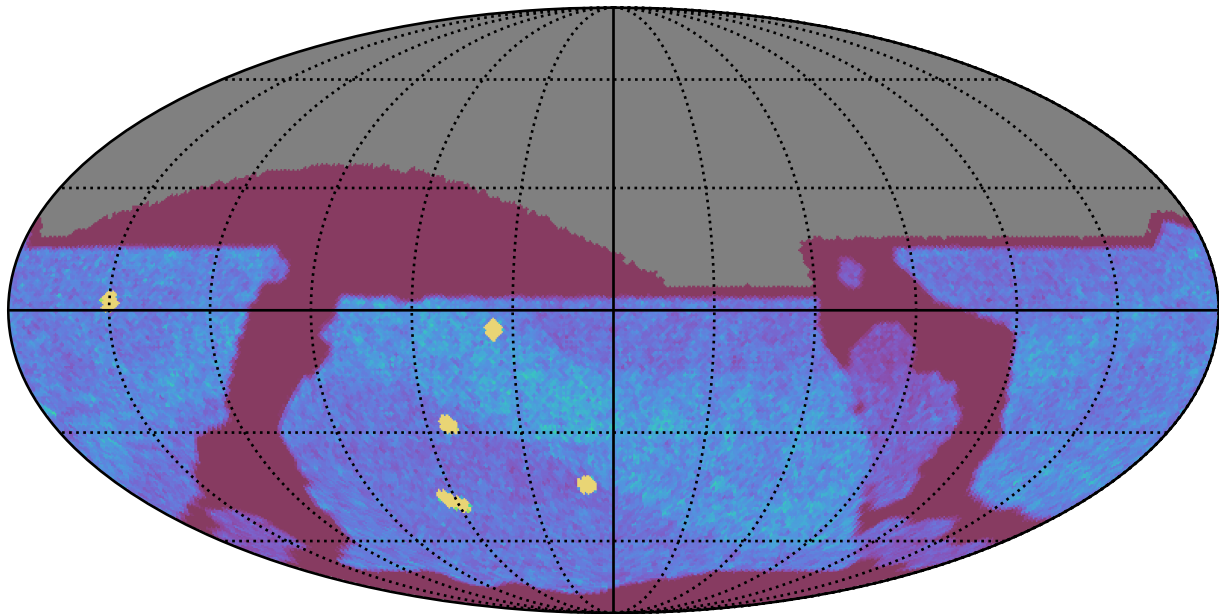
ddf_acor_sf30_lsf40_lsr10_v3.4_10yrs All sky z band: NVisits
