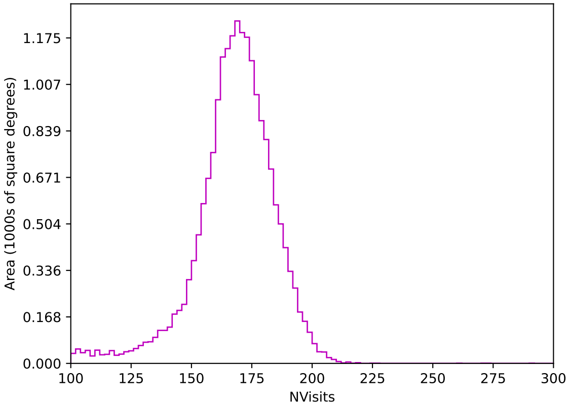
ddf_acor_sf30_lsf40_lsr10_v3.4_10yrs All sky z band: NVisits
